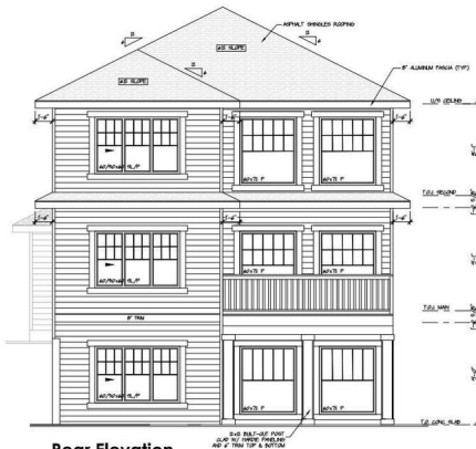
Rear Elevation
